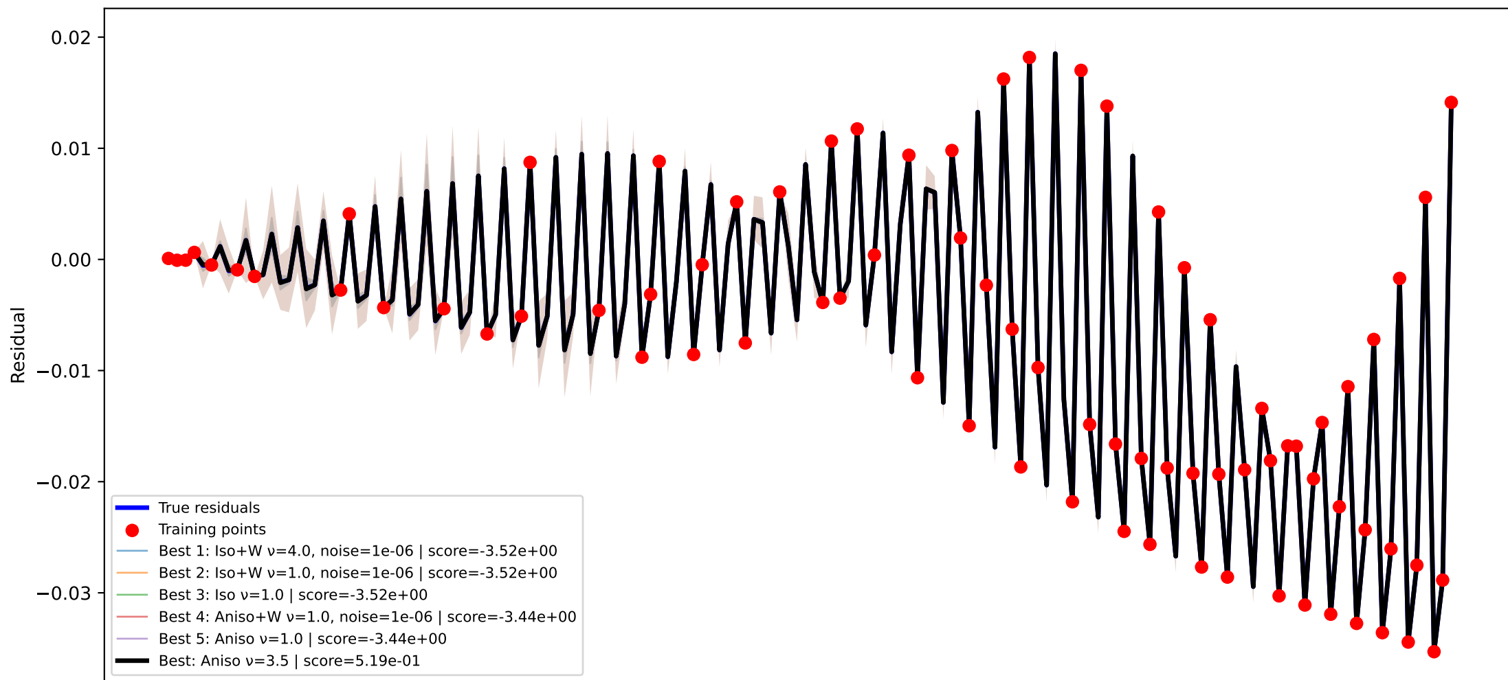
GPR kernel comparison node=39 RMSE=1.272e-05, train RMSE=5.759e-10
